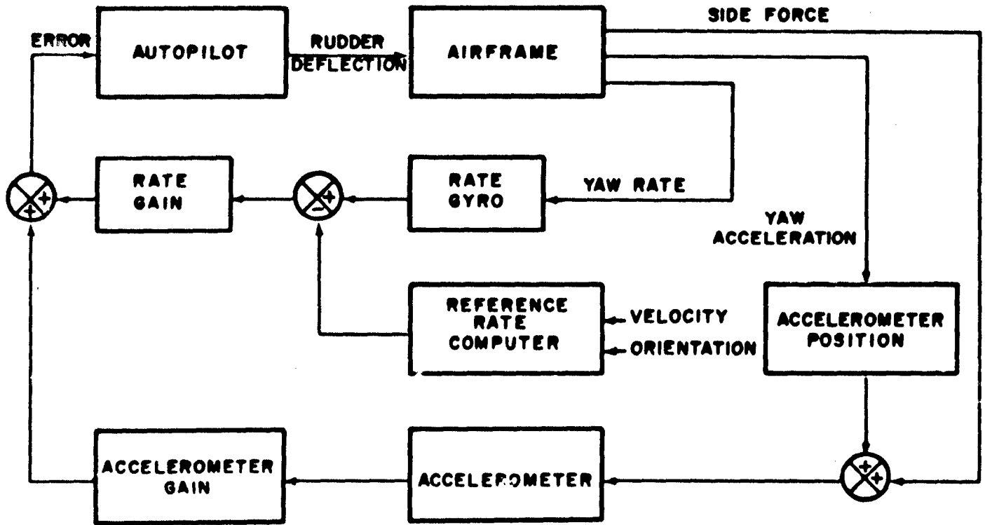
Figure 55. Yaw Control System with Accelerometer for Turn Coordination
