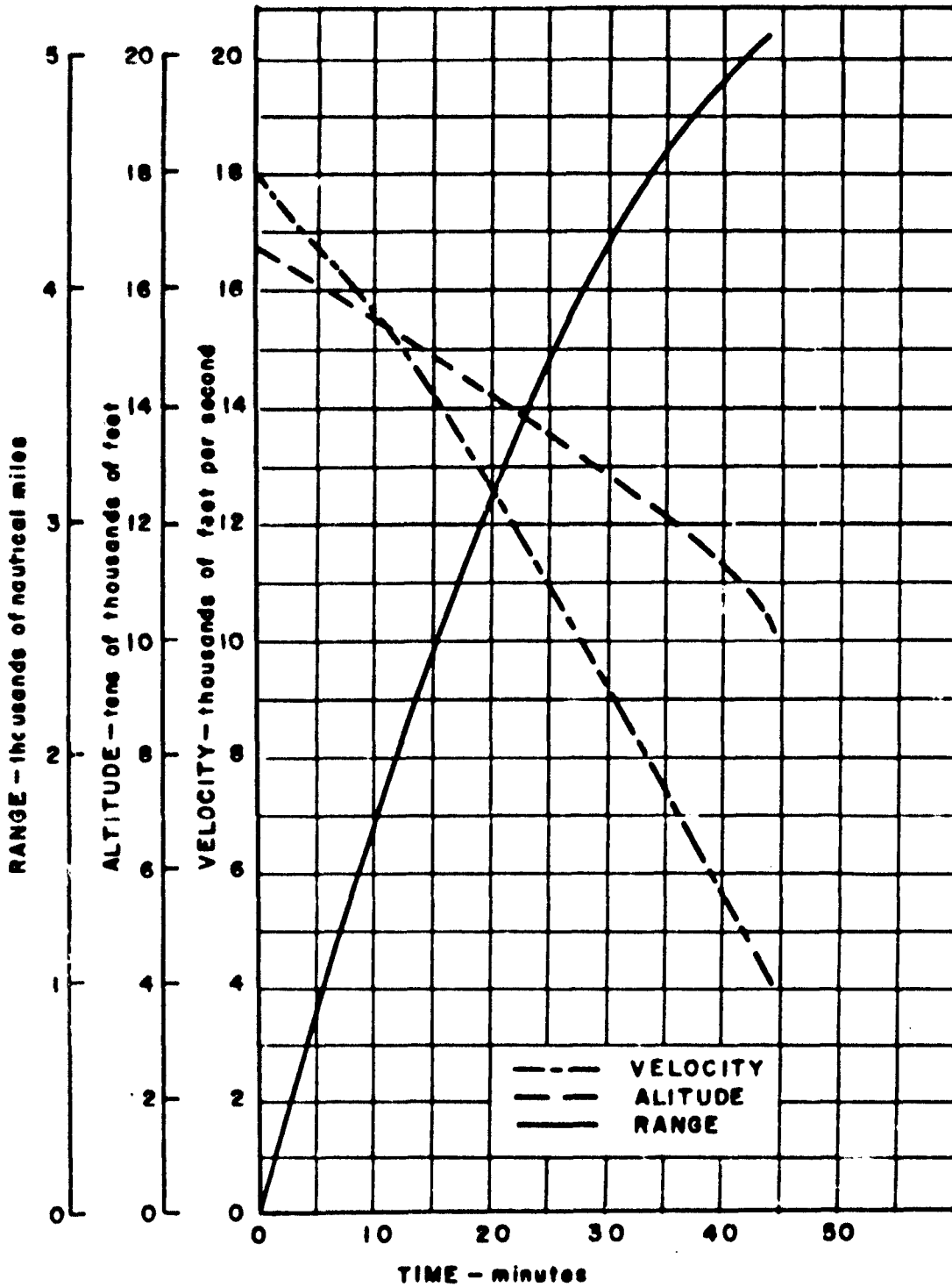
Figure 2. Typical Flight Profile - Glide Phase
