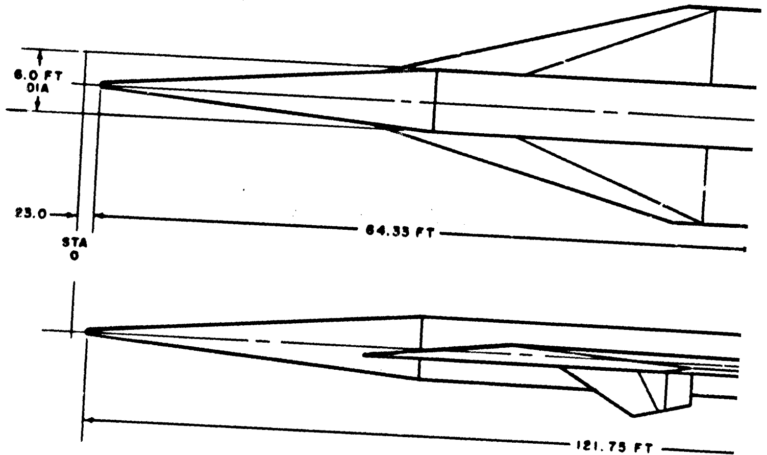
Figure 6. Typical Configuration
