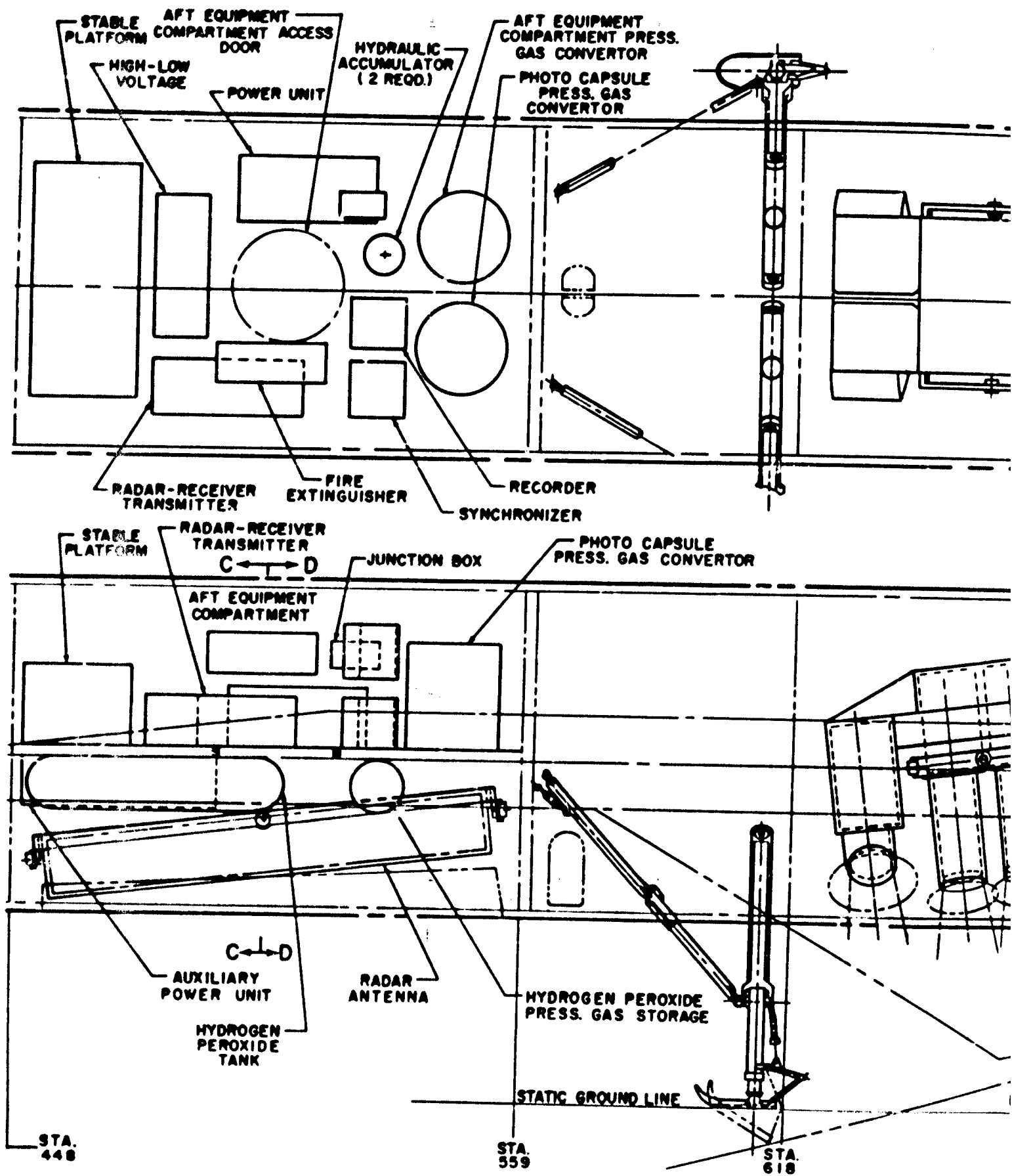
Figure 7. Inboard
