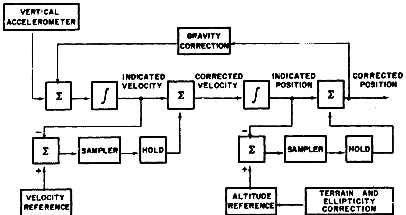
Figure 47. Inertial Vertical Instrumentation with Discrete Velocity and Position Corrections
