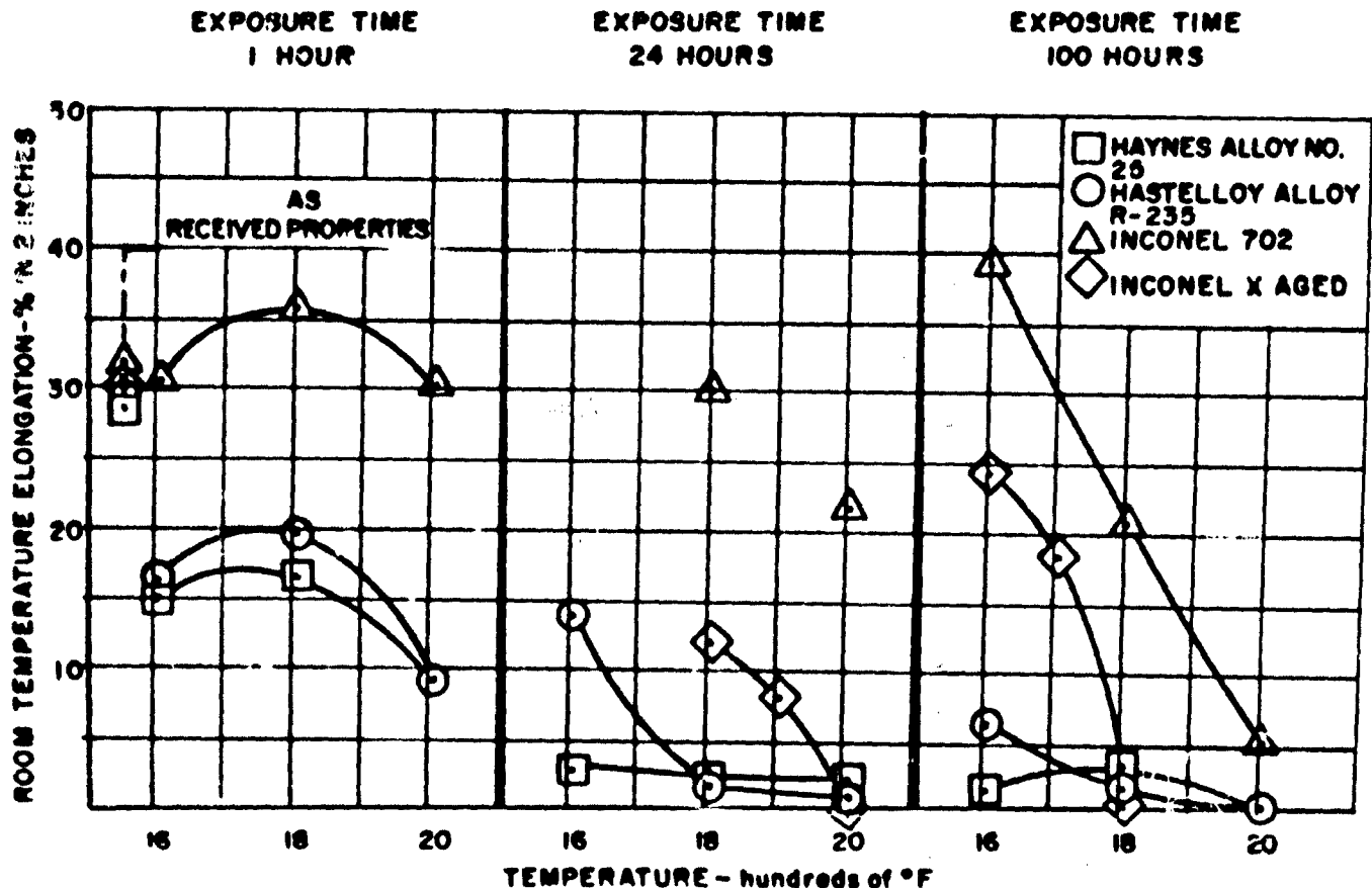
Figure 25. Room Temperature Elongation vs Temperature for Various Exposure Times - Air Atmosphere
