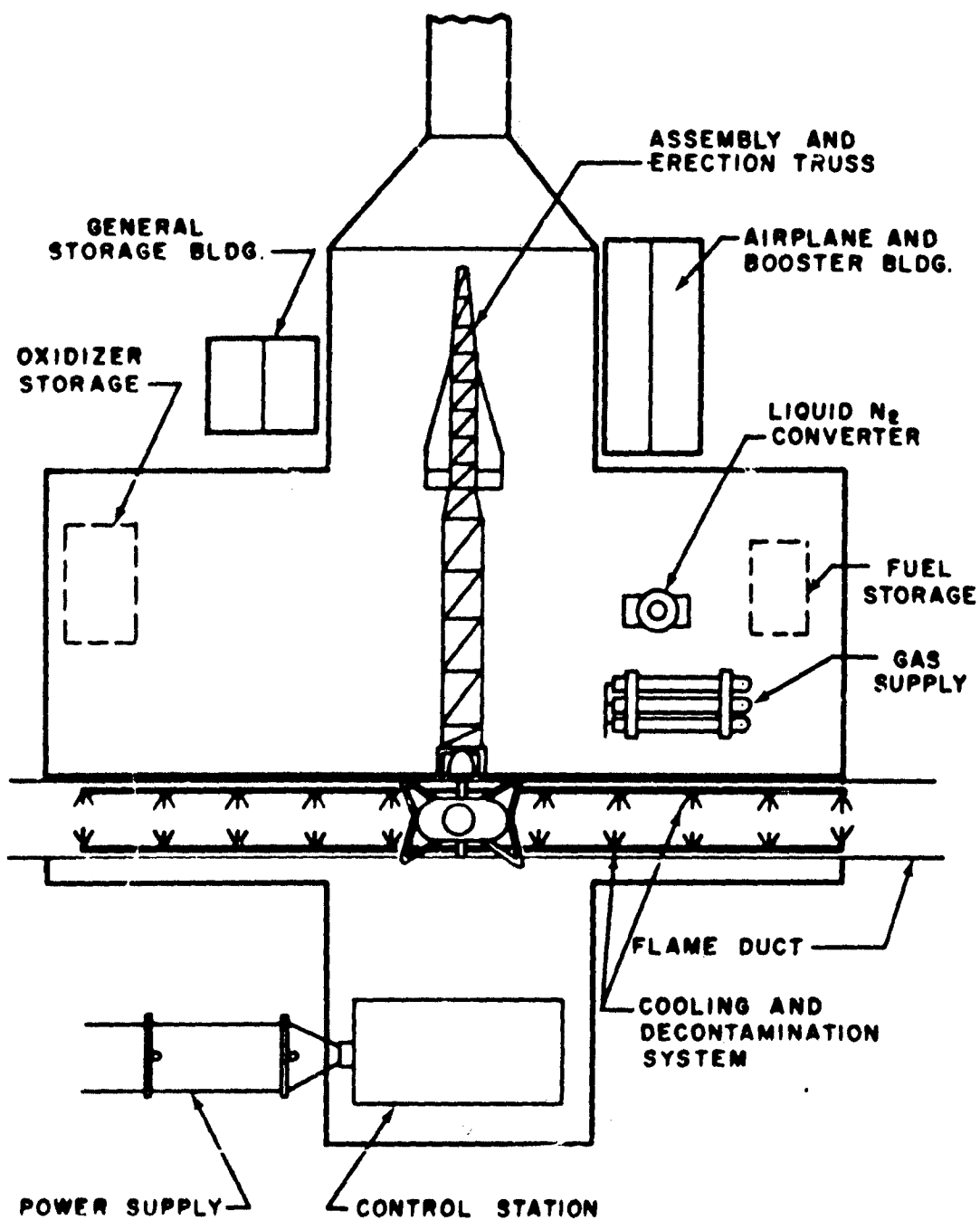
Figure 61. Rocket Test Facility
