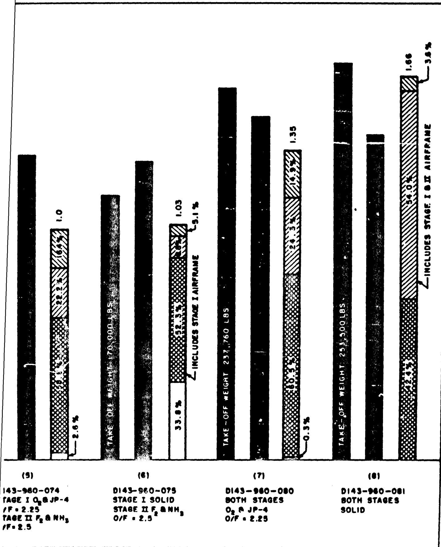
Figure 5. Propellant Evaluation
