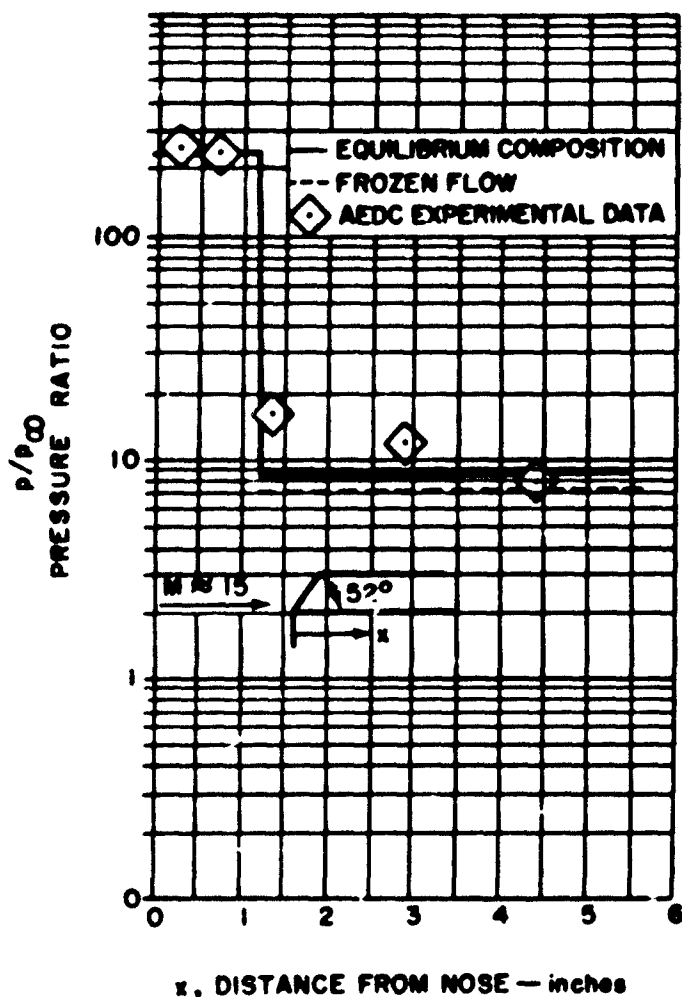
Figure 42. Pressure Distribution on Wedge-Plate Combination
