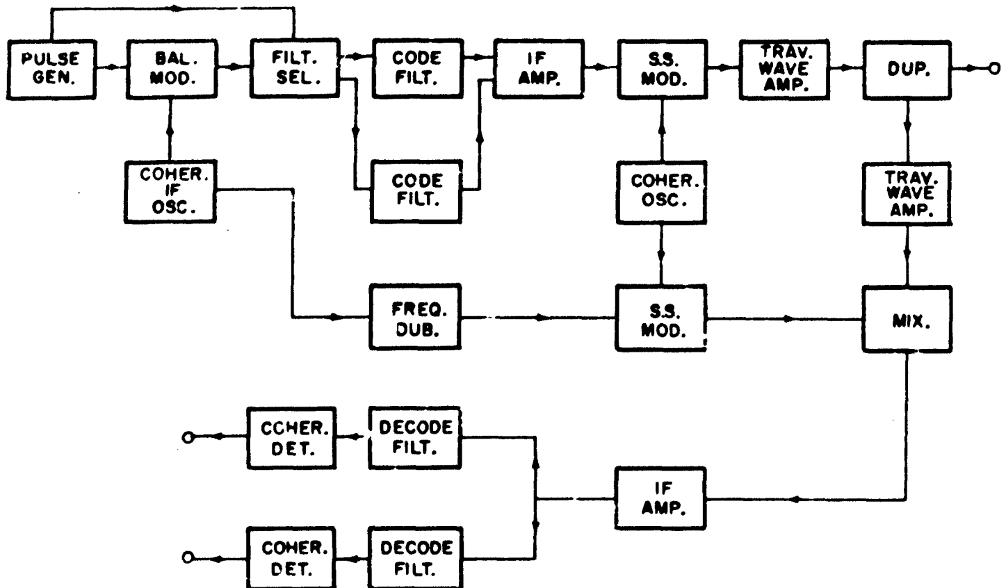
Figure 57. Chirp System
