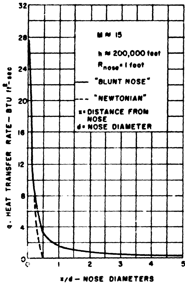
Figure 44. Theoretical Influence of "Blunt Nose Effect" on Heat Transfer Rate
