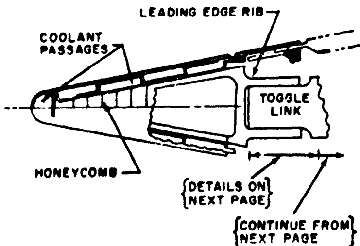
Figure 10. Leading Edge Design
