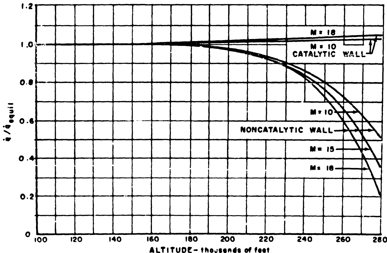
Figure 46. Nonequilibrium Stagnation Point Heat Transfer Variation with Flight Condition
